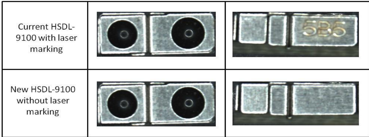
Figure 1: Comparison of the current HSDL-9100 with laser marking and new HSDL-9100 without laser marking.
